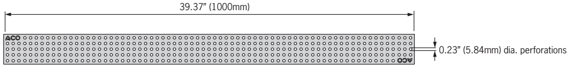
Plan view
